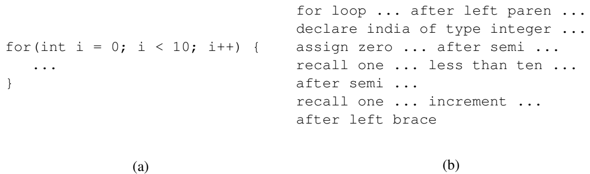
Figure 1.1: To get the for loop in (a), a VoiceCode user speaks the commands found in (b).
