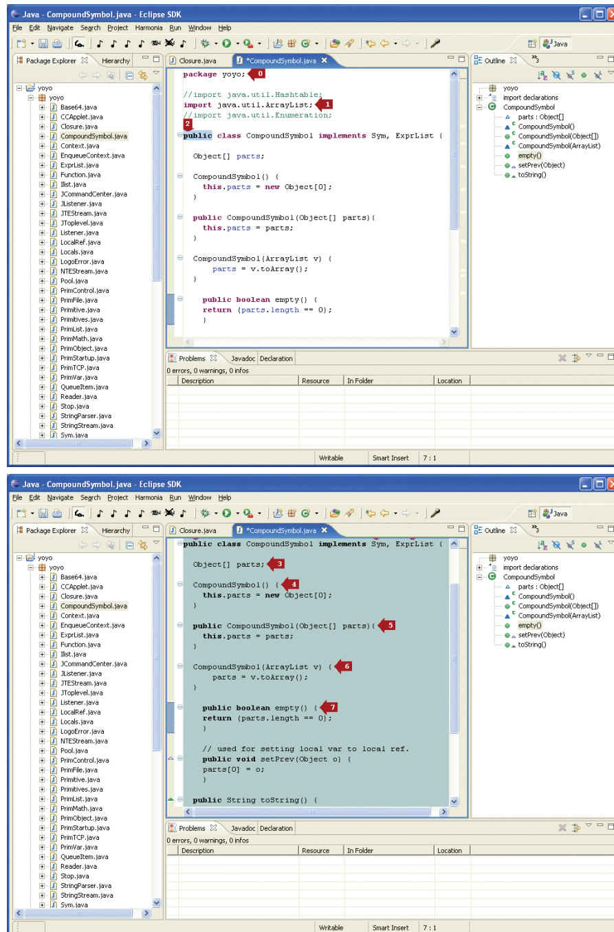
Figure 7.3: Part (a) shows Context-Sensitive Mouse Grid just after being invoked. Three arrows label the top-level structures in the file. Part (b) shows the same file after the number 2 (the class definition) has been picked. The entire class has been highlighted, and new arrows appear on the structural elements of the class that can be chosen next.
